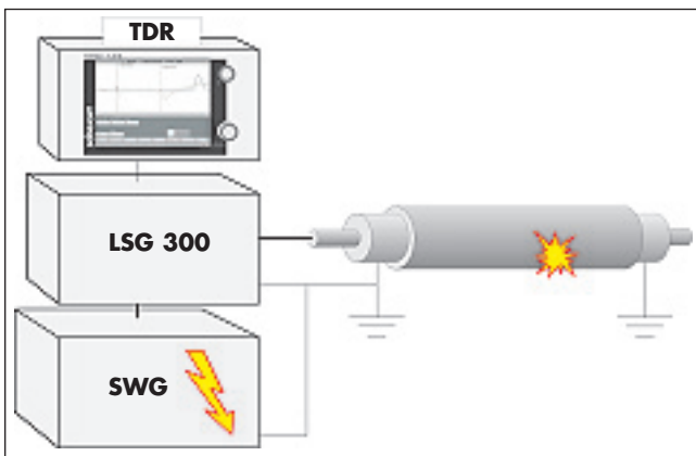
Fig. 1: Instrument configuration for the Arc Reflection Method (ARM)
